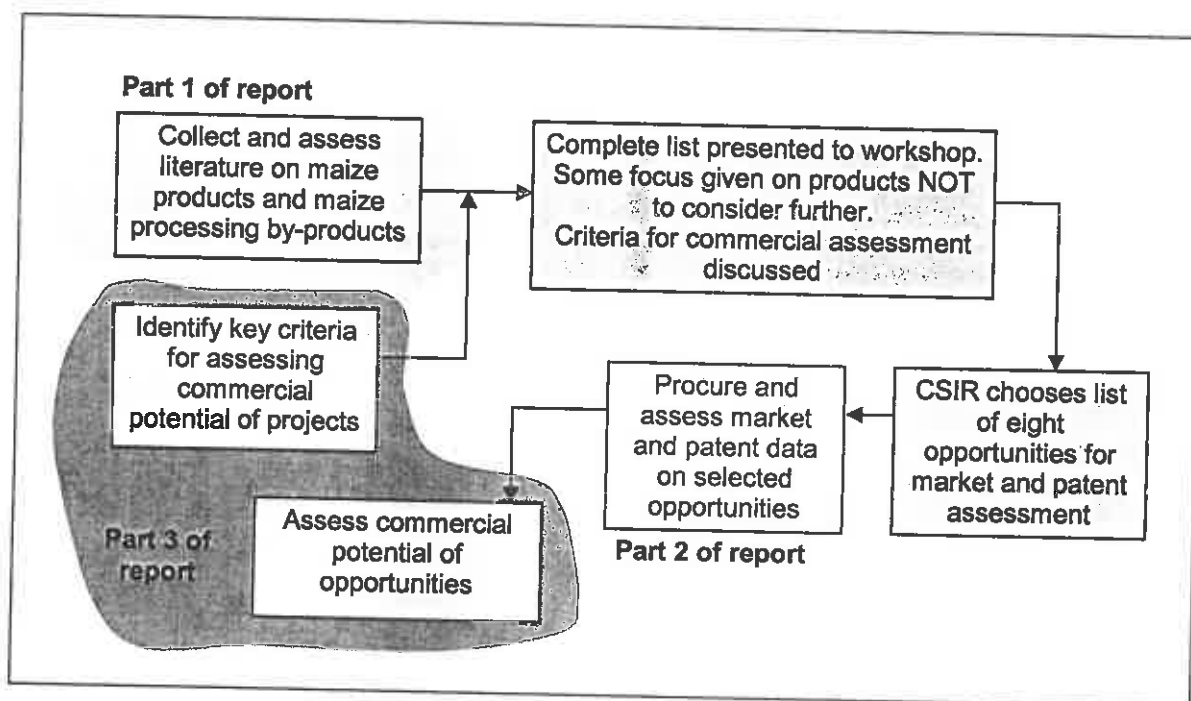
Figure 1: Methodology followed
