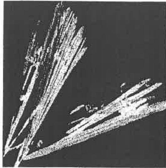
Fig. 4. Crystals of biotechnologic vanillin in polarized light (x200).
